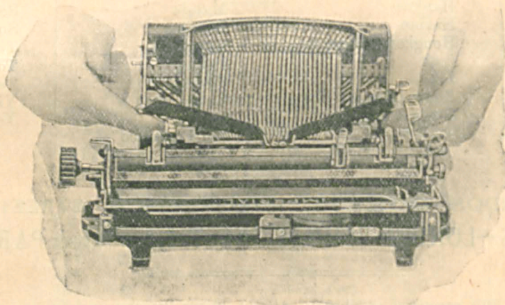
STANDARD MODEL No. 12.
