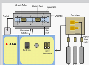
Fig 1. Schematic of TM-CVD for CNTs production
